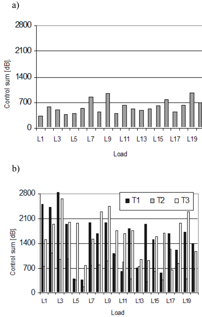
Fig. 4. Control sums for motor under different loads with bearings: a) faultless, b) damaged (T1, T2, T3).
