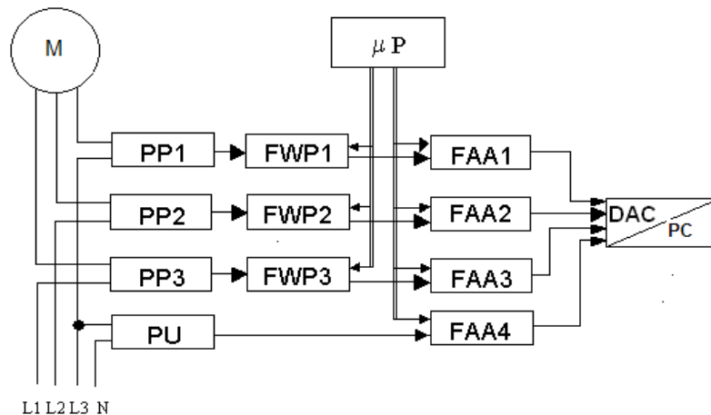
Fig. 2. Current measurement system for induction motor (where: M – induction motor; \mu P – microprocessor; PP1– PP3 – transducers for current measurements; PU – transducer for voltage measurements; FAA1- FAA4 – antialiasing filters; FWP1-FWP4 – narrow band filters; A/D – data acquisition card; PC – computer).
