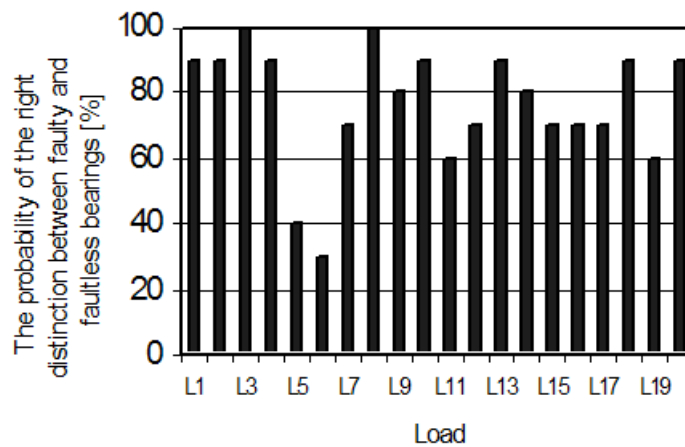
Fig. 5. The probability of the right distinction between faulty and faultless bearings.
